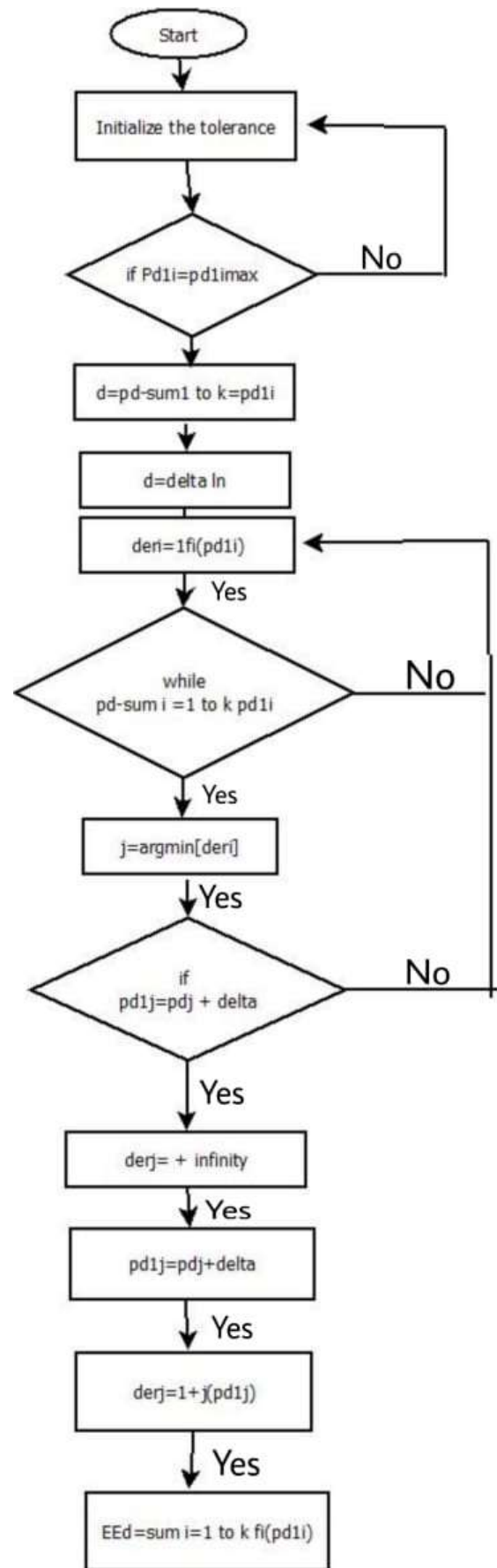
Figure 3: Flowchart for Proposed Derivative method
