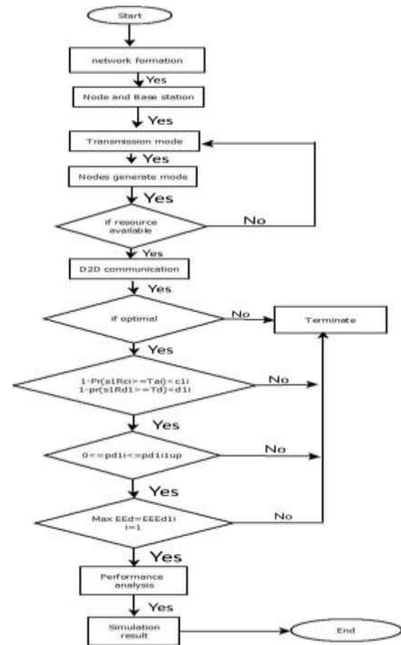
Figure 2: Flowchart for Branch and Bound
